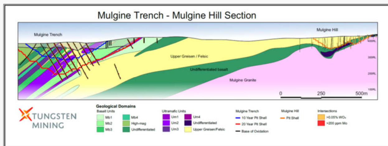
Figure 4: Interpreted geological domains (and sub-domains) at Mt Mulgine. Possible relationship / connectivity between the Mulgine Trench and Mulgine Hill deposits has been clarified for the first time.
