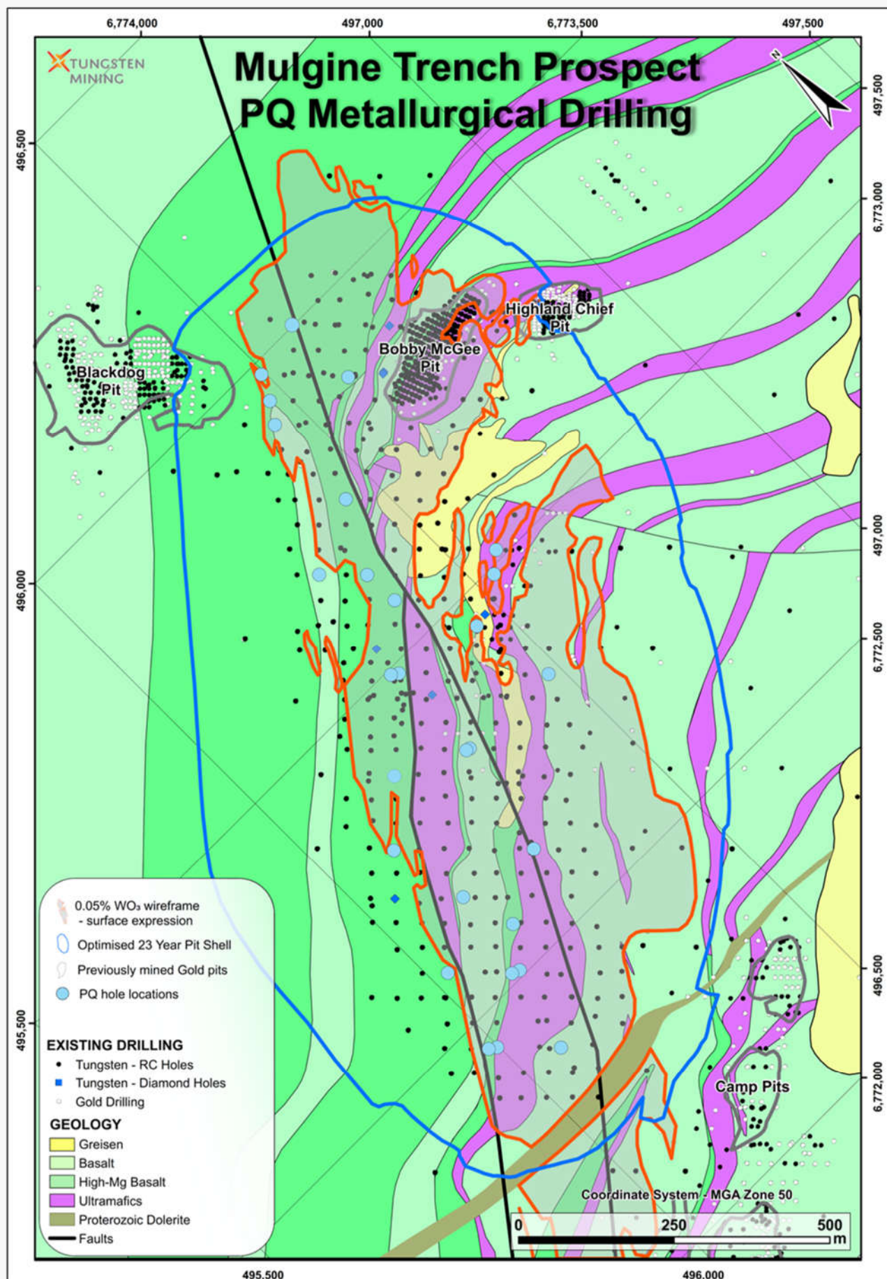
Figure 6: Location of PQ drilling (blue circles) on Mulgine Trench surface geology.
