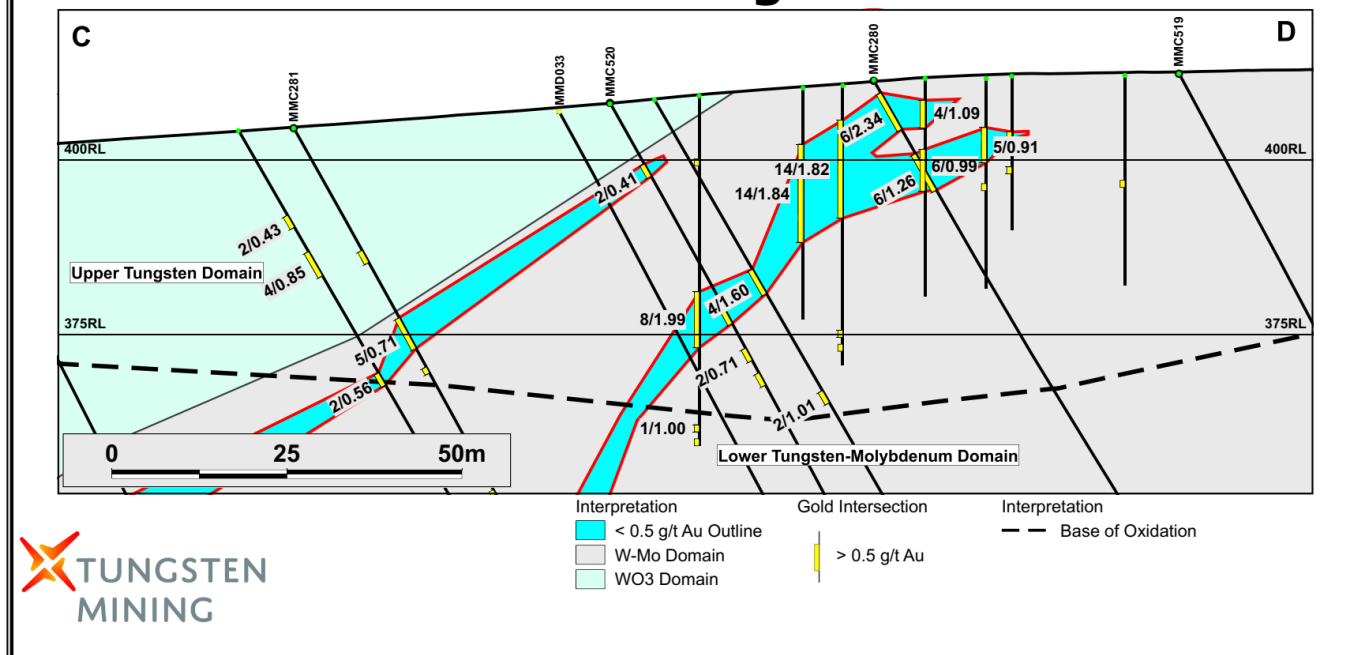
Figure 4. Section C-D showing supergene gold mineralisation in the centre of the Mulgine Trench oxide gold target.
